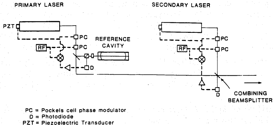
VI-4: A method to increase optical power by coherent addition of lasers.
