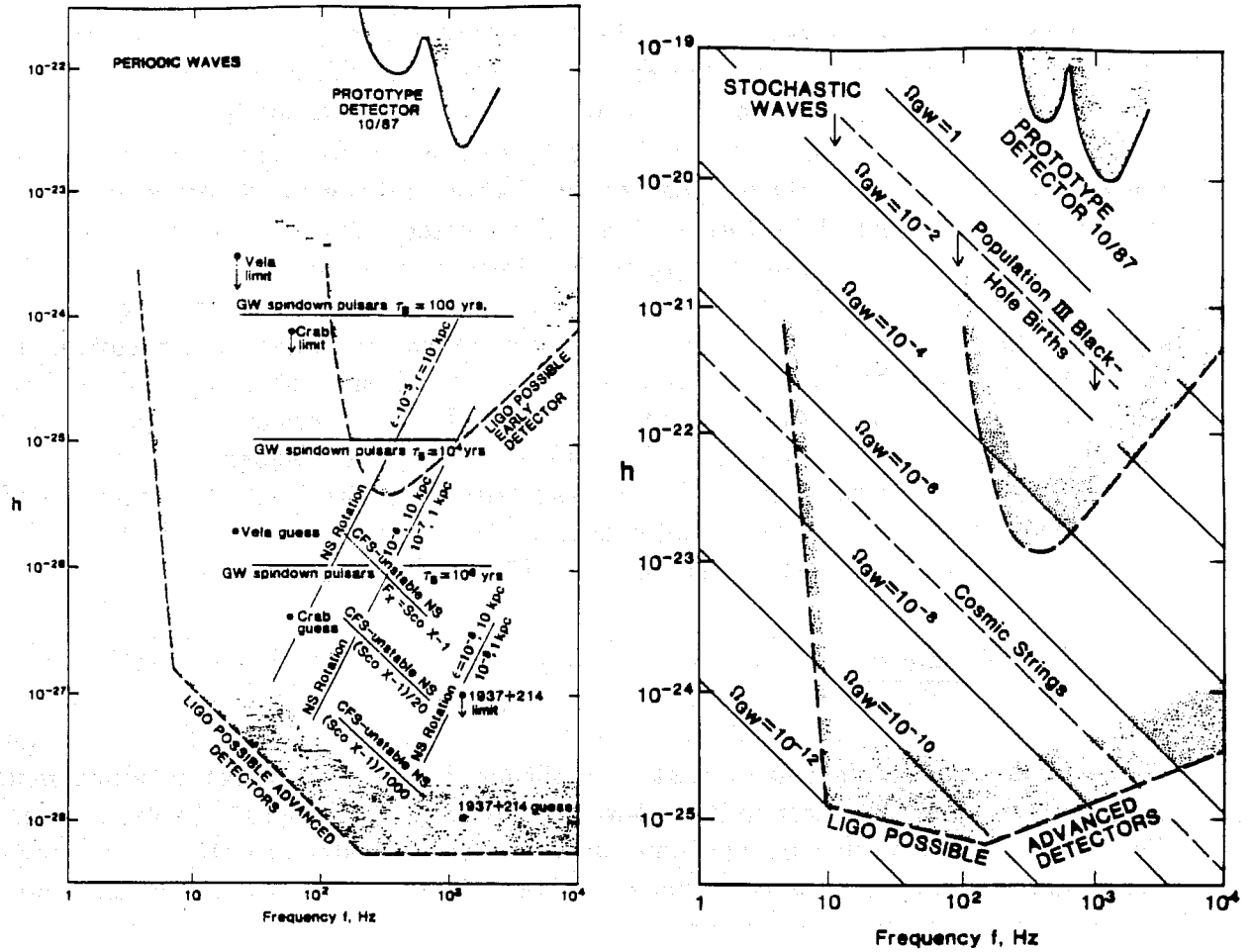
Figure A-4b,c Same as Figure A-4a, but for periodic waves (b), and for stochastic background waves (c). In both figures the detectors are assumed to use an integration time of 10^7 seconds.
