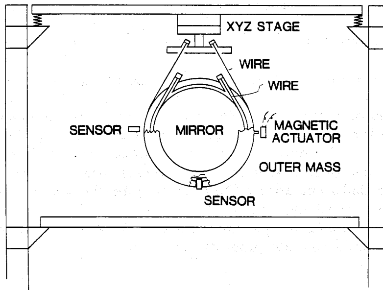
Figure V-9: A schematic diagram of the multiple suspension system under development for the 5-meter prototype.
