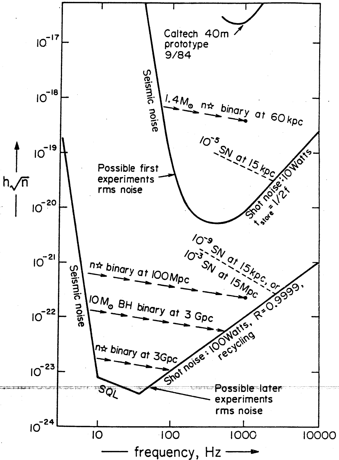
Figure 2.2 Comparison of predicted gravity wave strength for burst sources with possible detector sensitivities. See text for details about source and detector assumptions.
