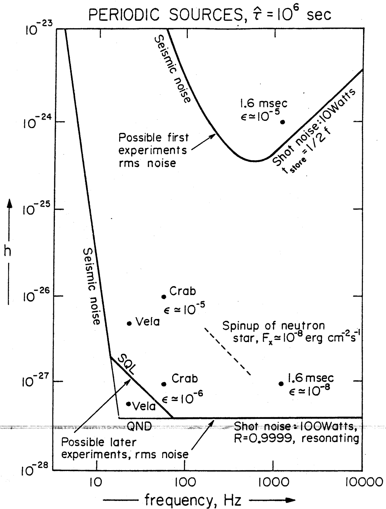
Figure 2.3 Comparison of predicted gravity wave strength for periodic sources with possible detector sensitivities. See text for details about source and detector assumptions.
