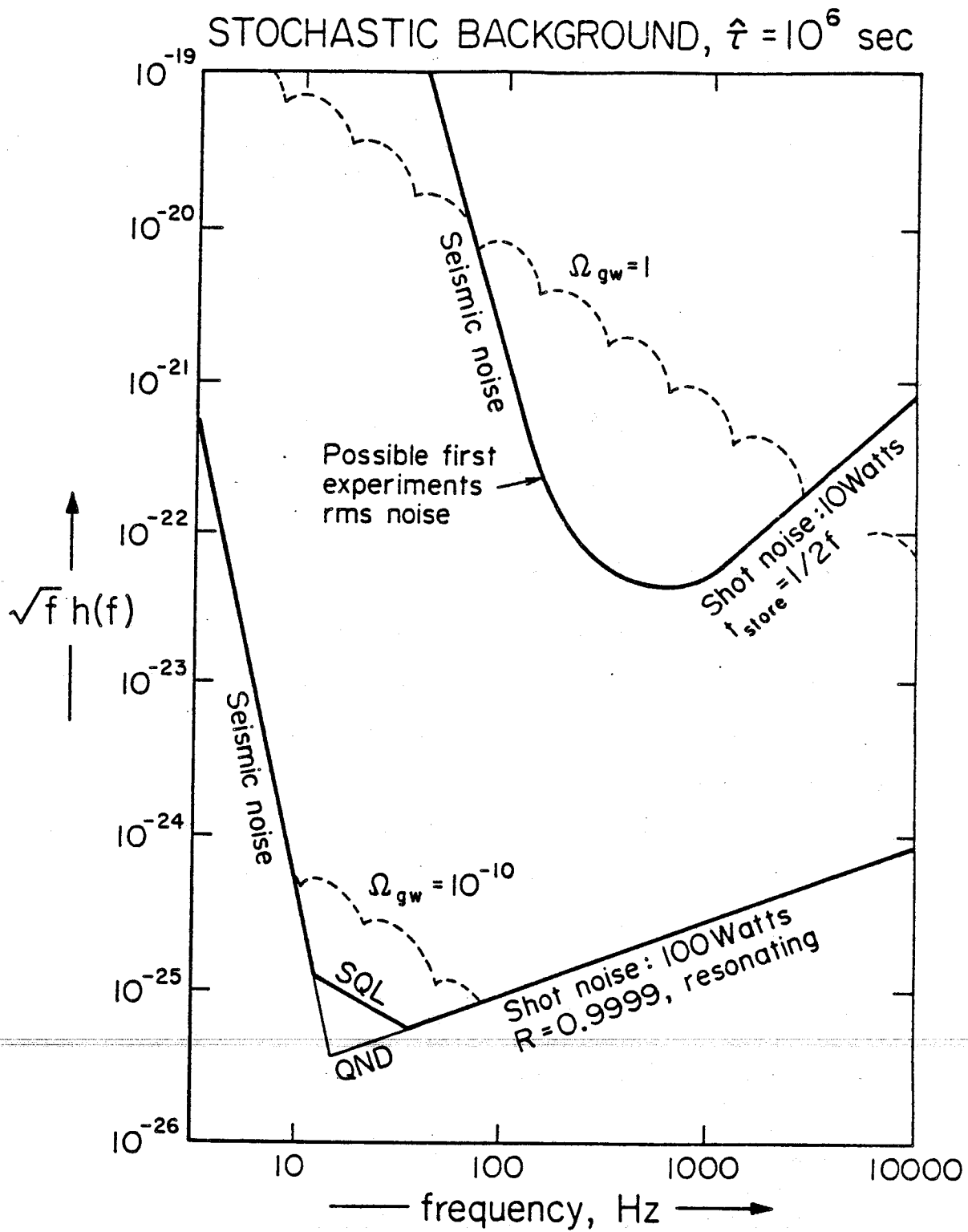
Figure 2.4 Comparison of possible strength of stochastic gravity wave backgrounds with possible detector sensitivities. See text for details about source and detector assumptions.
