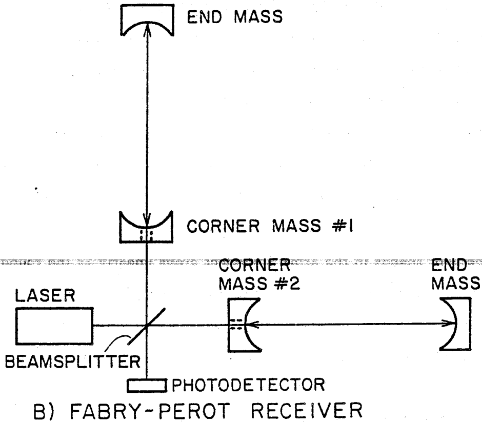
Figure 2.1 Simplified diagrams of Michelson and Fabry-Perot gravitational wave receivers. (In the lower diagram the corner mass is shown as two parts - a method for avoiding the thermal noise associated with low frequency resonances of a complex mass).
