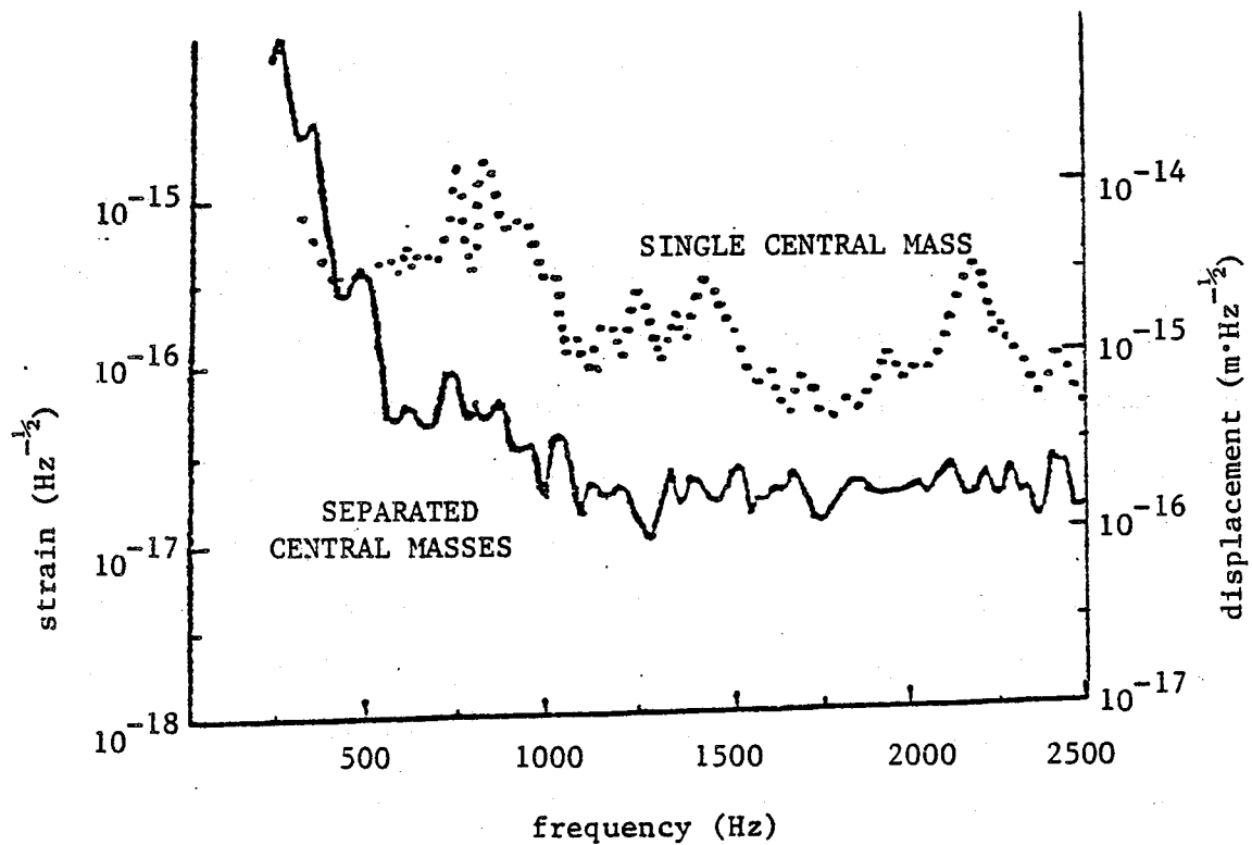
Figure 3.7 Noise spectra of the Glasgow 10 m prototype antenna. These spectra, which are calibrated in both strain ( \text{Hz}^{-1/2} ) and in displacement ( \text{m} \cdot \text{Hz}^{-1/2} ), show the improvement obtained by placing the cavity mirrors on separate, low-noise masses.
