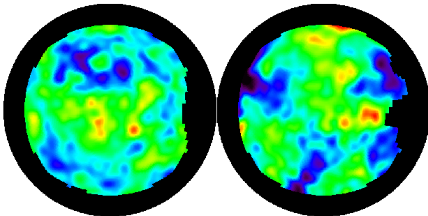
North Galactic Hemisphere
