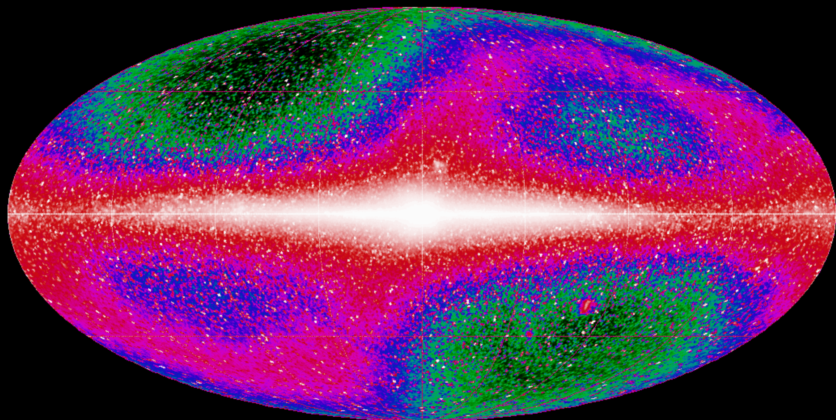
DIRBE 3.5 MICRONS, MJY/SR
